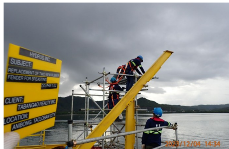
Installation of A-Frame
